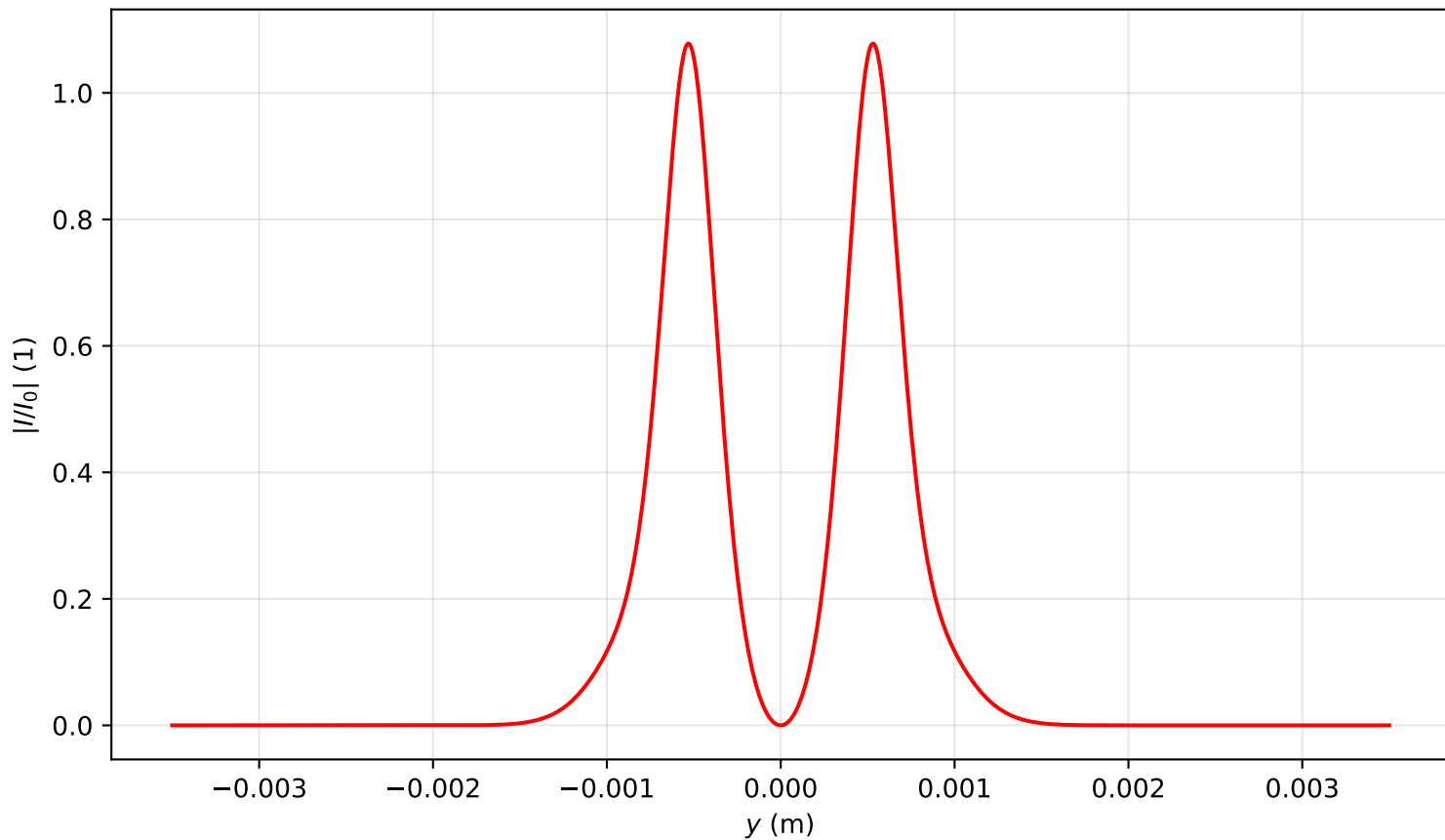
Intensity profile I(x=0, y, z=0.557)/I_0 , P_{in}=5.0P_{cr} , artificial time
